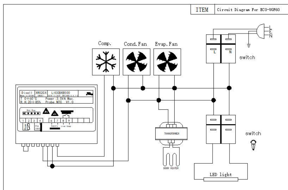
Photo 2 - Circuit diagram:
