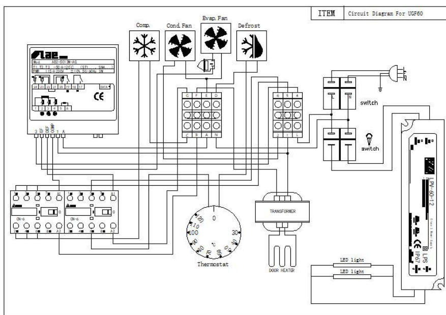
Photo 2 - Circuit diagram:
