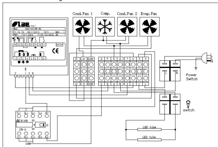
Photo 2 - Circuit diagram:
